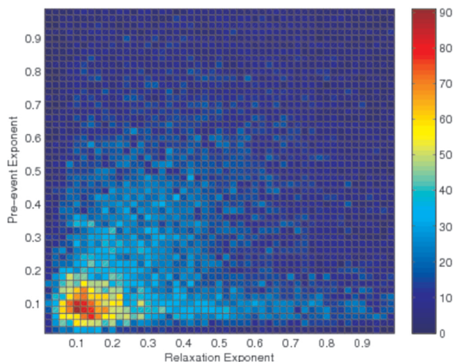
Fig. 6. 2D Histogram of the pre-event and relaxation exponents for the 54,312 time-series whose preevent exponent is defined. The highest density of points cluster near p = 0.15 . This not only provides evidence that the prevent and relaxation exponents are equal within the precision of our analysis algorithm, but provides independent support that we have correctly identified the endogenous-critical class, since this class has the largest number of videos satisfying the predicted exponent equality.
